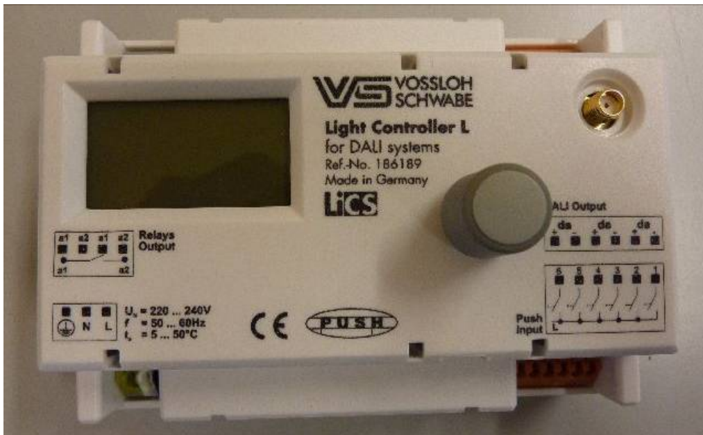
Light controller
